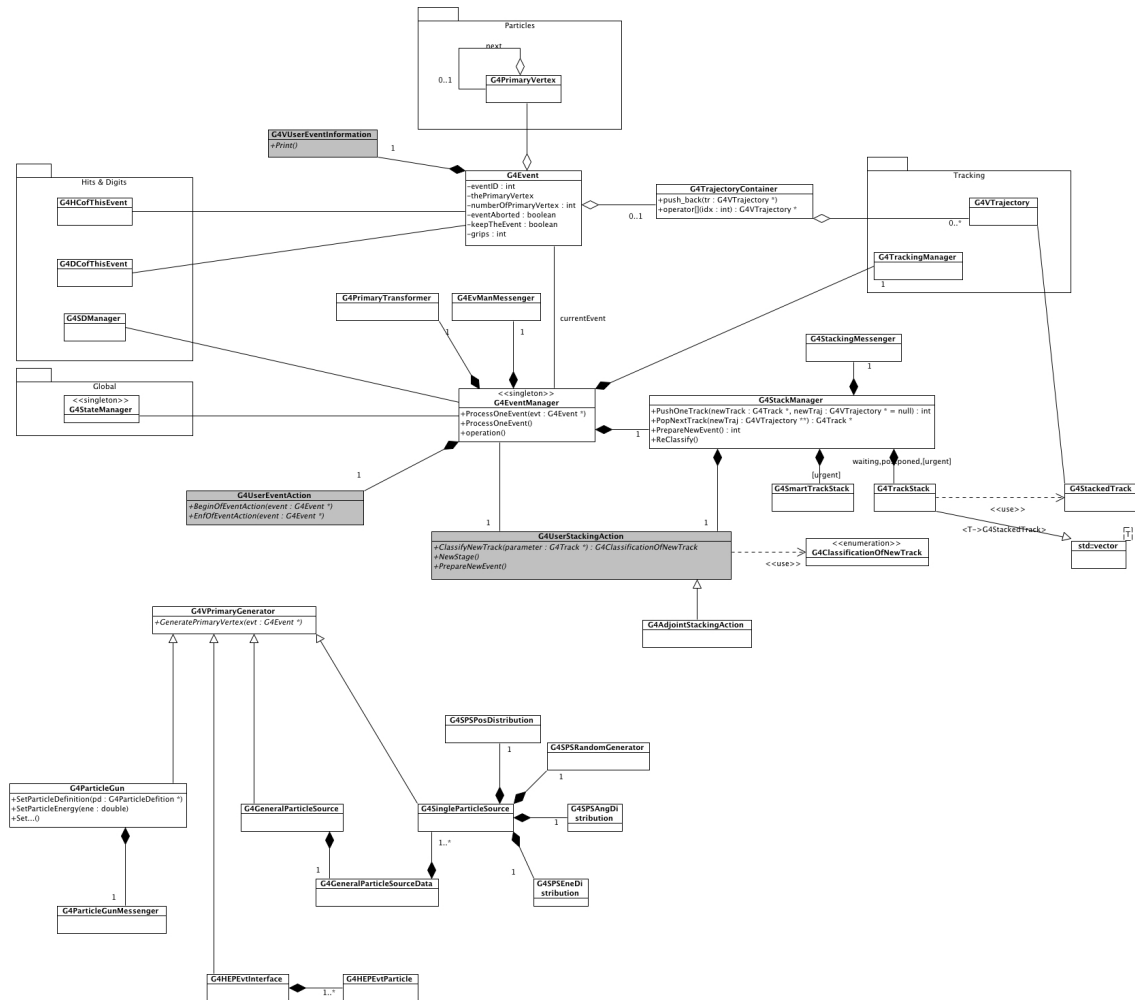
Fig. 2.3: Event Category UML Diagram. Classes in grey are to be sub-classed by user.
