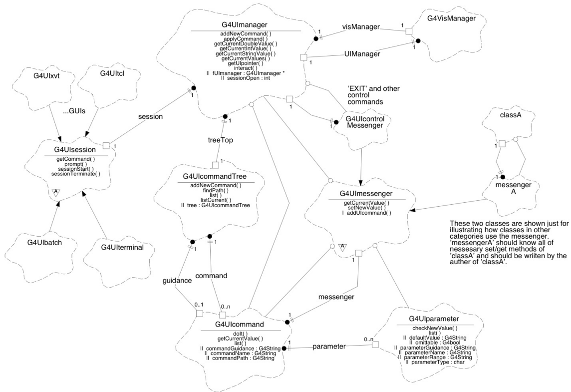
Fig. 2.25: Overview of intercom classes
