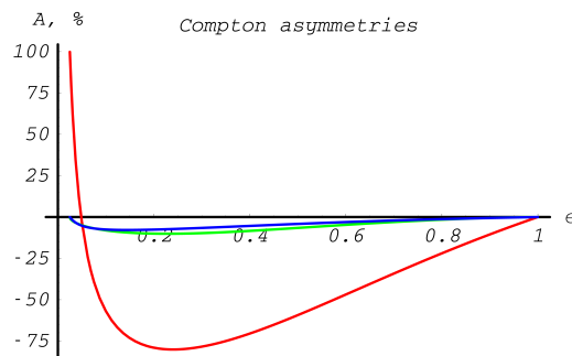
Fig. 13.20: Compton scattering differential cross section asymmetries in%. Red line corresponds to the asymmetry due to circular photon and longitudinal electron initial state polarization, green line – due to circular photon and transverse electron initial state polarization, blue line – due to linear photon and transverse electron initial state polarization.
