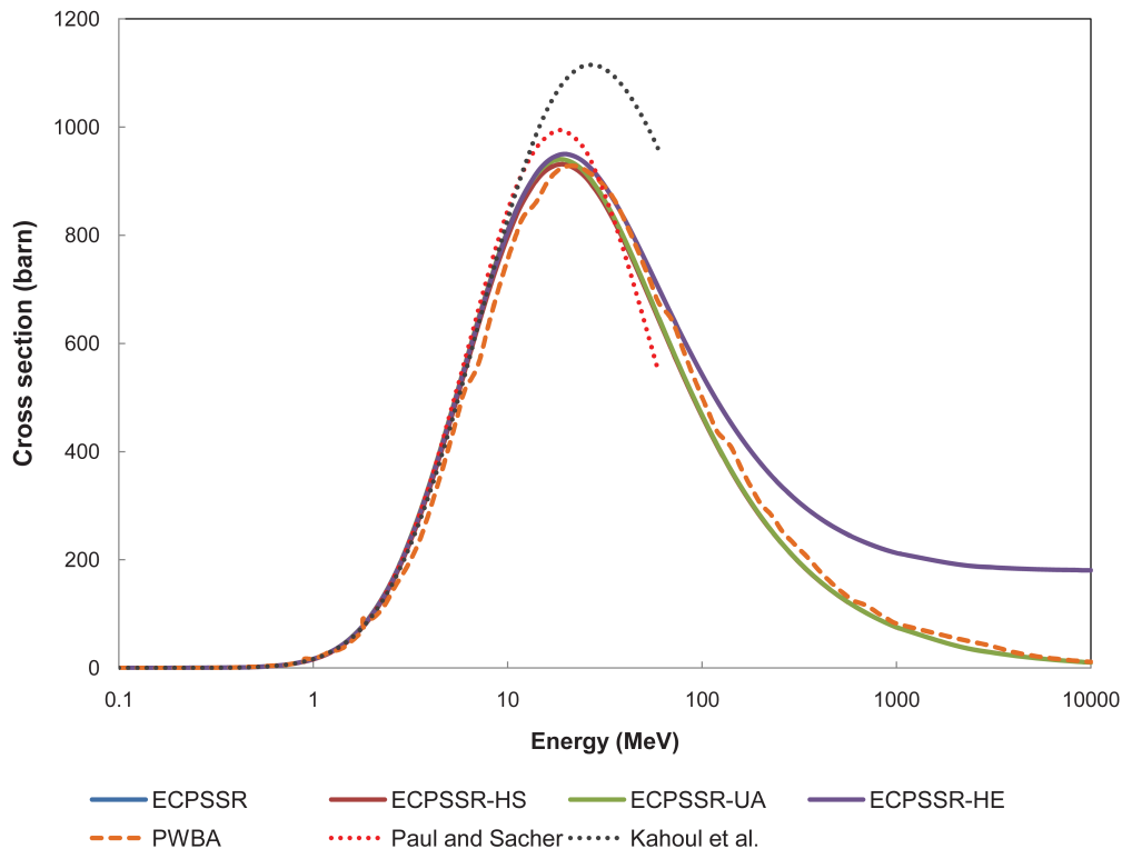
Fig. 9.1: Cross section for the ionisation of copper K shell by proton impact according to the various implemented modeling options: ECPSSR model, ECPSSR model with “united atom” (UA) approximation, Hartree-Slater (HS) corrections and specialized for high energies (HE); plane wave Born approximation (PWBA); empirical models by Paul and Sacher and Kahoul et al. The curves reproducing some of the model implementations can be hardly distinguished in the plot due to their similarity.
