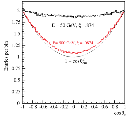
Fig. 10.7: Generated histograms with 10^6 entries each and the expected \cos \theta_{\text{cm}} distributions (dashed lines) at E = 50 and 500 GeV positron energy in the lab frame. The asymptotic 1 + \cos^2 \theta_{\text{cm}} distribution valid for E \rightarrow \infty is shown as dotted line.
