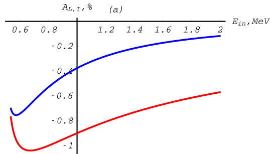
Fig. 13.4: Bhabha total cross section asymmetries depending on the total energy of the incoming positron, with a cut-off T_{cut} = 1\text{keV} . Transverse asymmetry is plotted in blue, longitudinal asymmetry in red. Between 0.5 MeV and 2 MeV.
